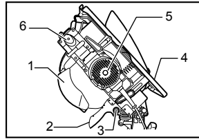
1. Lower blade guard A 2. Lower blade guard B 3. Clamping screw 4. Top table 5. Motor housing 6. Handle
