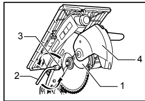
1. Center cover 2. Socket wrench 3. Hex bolt 4. Blade guard A
