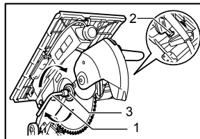
1. Socket wrench 2. Shaft lock 3. Hex bolt
