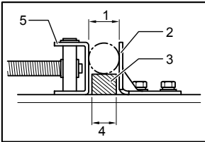
1. Diameter of workpiece 2. Guide plate 3. Spacer block 4. Width of spacer block 5. Vise
