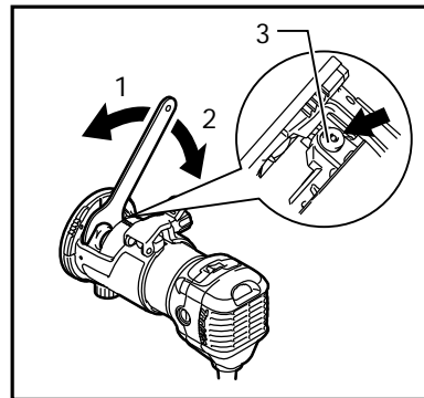
1. Tighten 2. Loosen 3. Shaft lock
